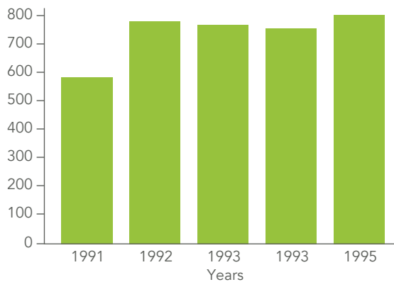
Figure 1. Mean cocoa yield response across fertilizer treatments over a five year period in Santander, Colombia.
